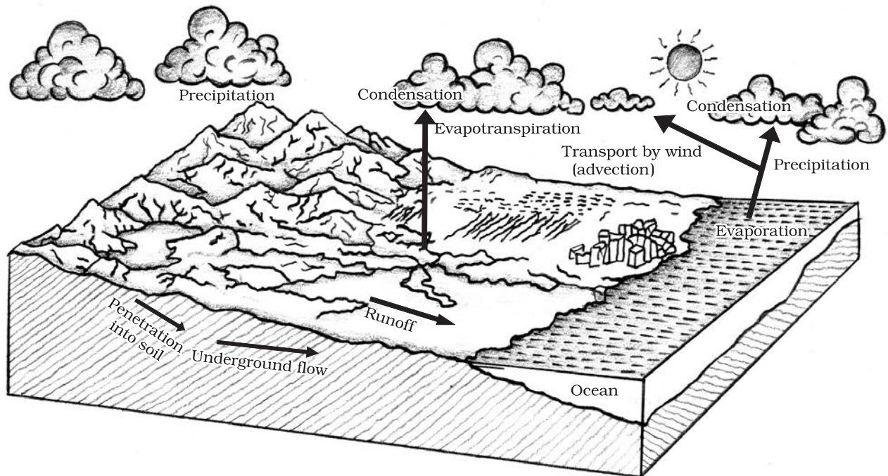
Figure 13.1 : Hydrological Cycle
